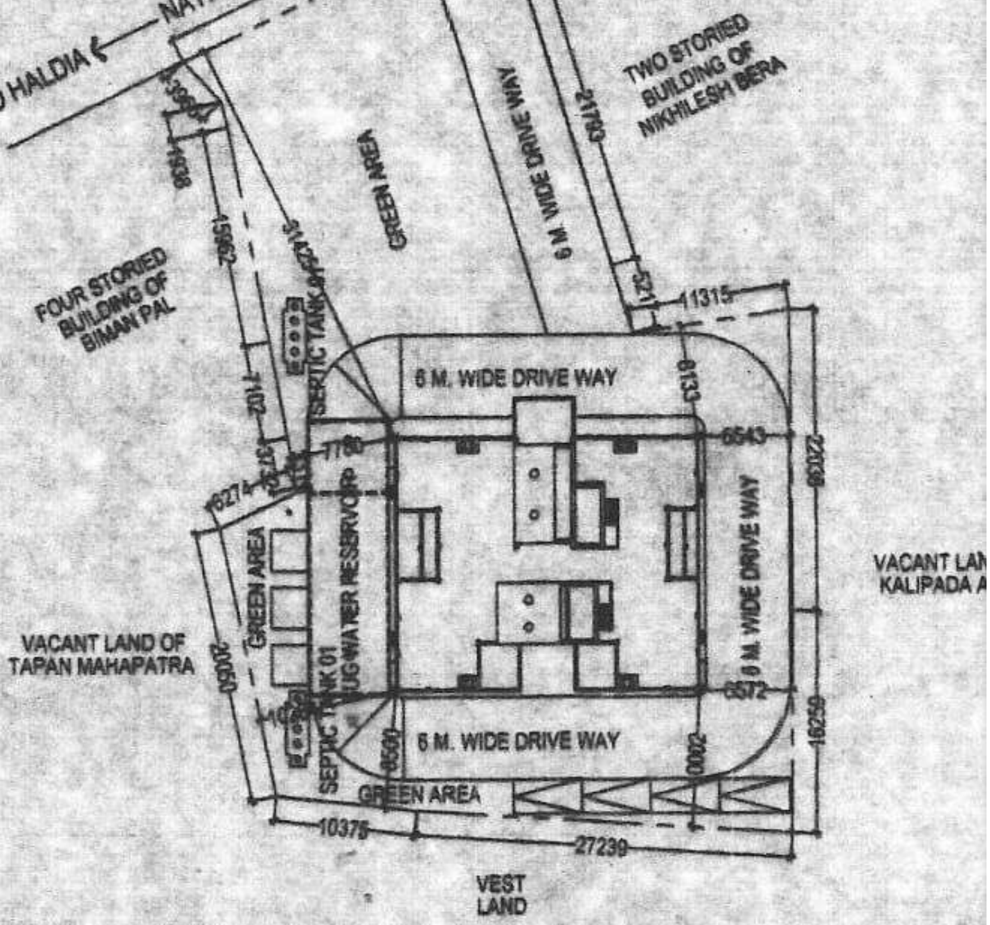
SITE PLAN SCALE- 1:600
